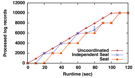
Fig. 11: Seal-based strategies, 10 ad servers.
