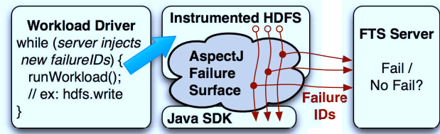
Figure 2: FTS Framework.
