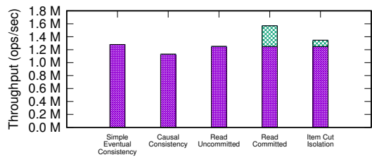
Fig. 10: Performance Across Consistency Levels
